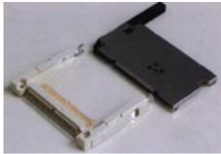
Compact Flash Type II Connector - 752D Positions: 50
