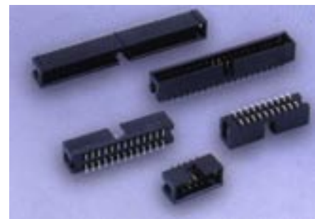
Box Header SMT 2.54mm - 302D Positions: 10 14 16 20 24 26 30 34 40 44 50 60 64
