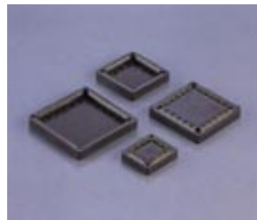
PLCC Socket SMT Type 1.27mm - 402D Positions: 20 28 32 44 52 68 84
