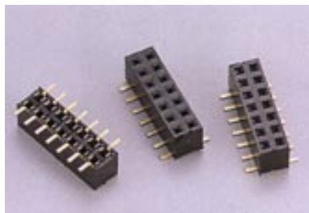
Female Header SMT 1.27mm x 2.54mm - 711D Positions: 10 ~ 120
