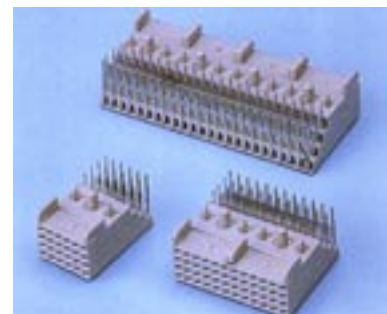
Future Bus R/A Female Solder Type (4x6, 4x12, 4x24, 4x48) - 609A
