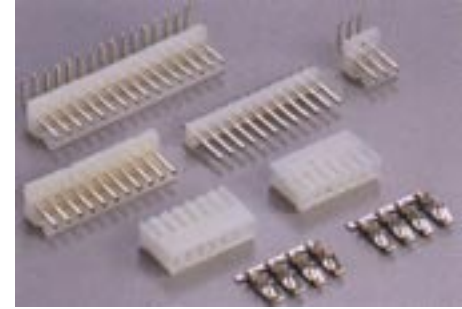
Wafer 3.96mm - 314A Crimp Terminal Housing 3.96mm - 315A Positions : 02 ~ 20 Crimp Contacts 3.96mm - 316A
